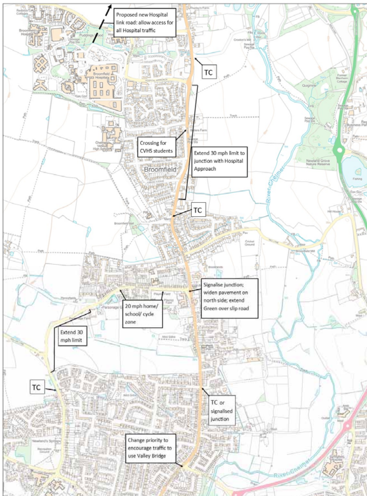
Fig. 30 – Current Neighbourhood Plan suggestions for traffic mitigation (larger scale maps at Appendix 7)
